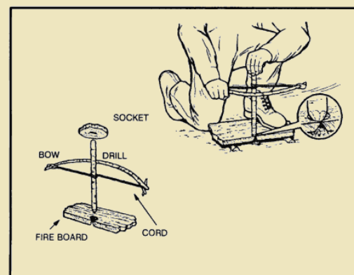
Figure 7-8. Bow and drill.
